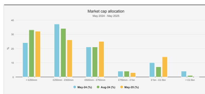
Fig.1: Market-Cap Allocation
